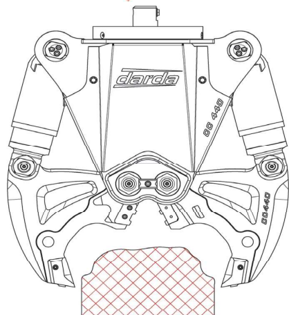
Crusher with standard tips
