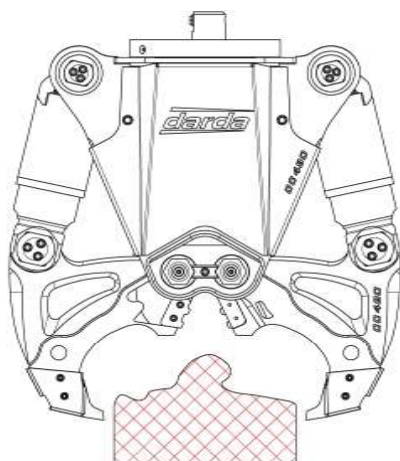
Crusher with standard tips
